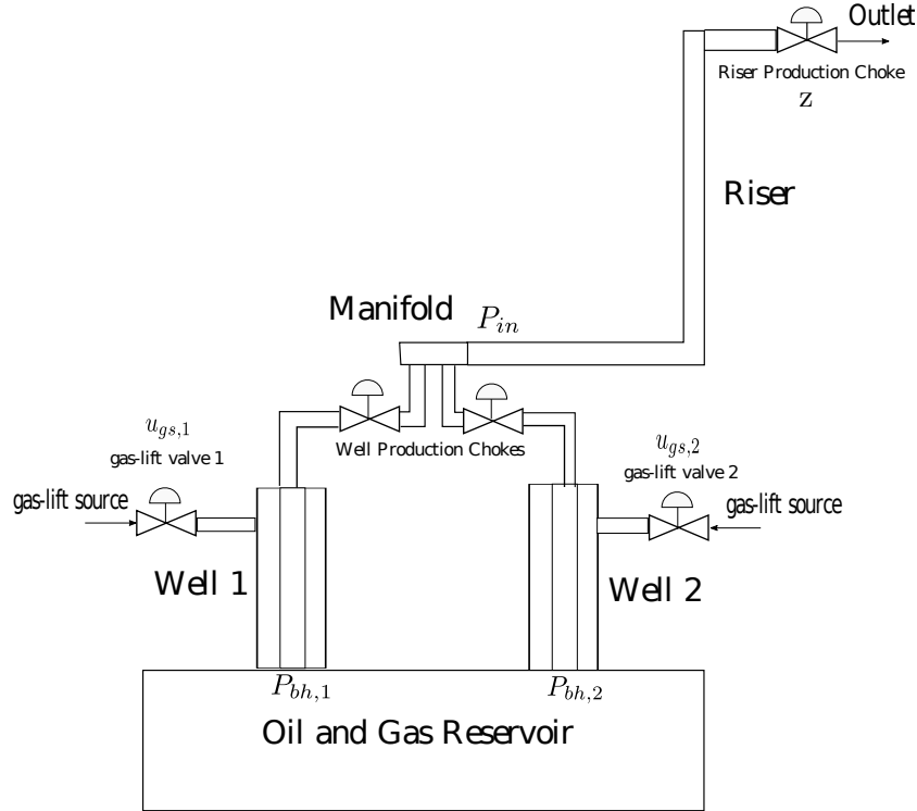
Figure 6: Representation of an oil platform containing two wells and one riser. From [20].
