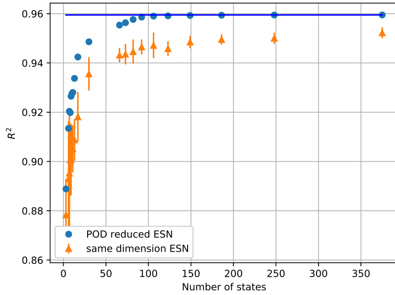
Figure 5: Experiment comparing a POD-reduced ESN (blue dots) with an ESN of equivalent size (to the reduced ESN) (orange triangles) for the 10th-order NARMA task. The POD reduction is applied on an ESN with 1,400 units in the reservoir. The horizontal axis is the number of states (units) of the reduced (full) network, while the vertical axis is the R^2 metric on the test set. The plot's blue horizontal line corresponds to the R^2 of the 1,400 units ESN.
