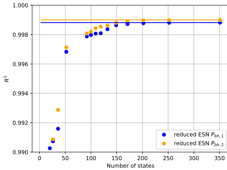
Figure 7: POD-ESN for a system identification task. The full ESN network has 1,400 neurons and was trained to model the platform with two wells and one riser. The x axis is the number of states of the reduced network, whereas the y axis is the R^2 metric on the test set for each output variable (bottom-hole pressures). The bottom-hole pressure of the first well is represented in blue, while the orange color denotes the bottom-hole pressure of the second well. The R^2 of the original network corresponds to the horizontal lines of the respective colors for comparison.
