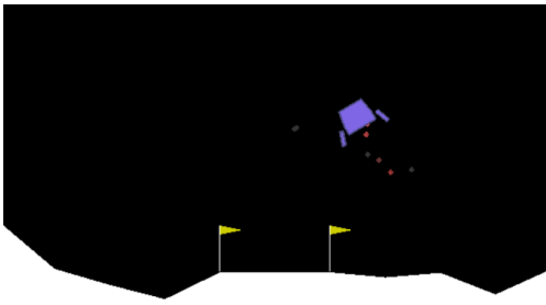
Fig. 2. LunarLanderContinuous-v2 Environment
